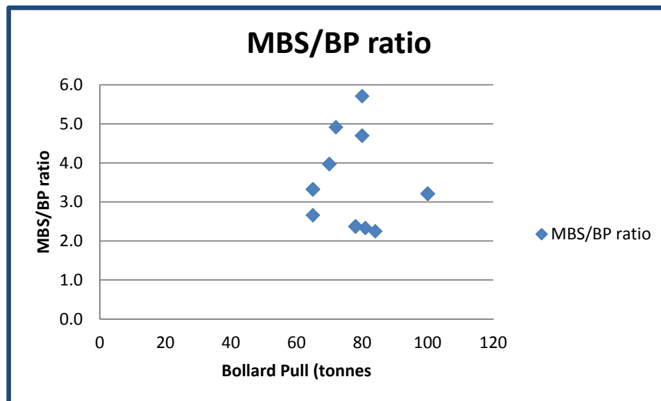
Figure 2.7 Ratio of Tug Thrust (Bollard Pull) to Mean Breaking Strength
