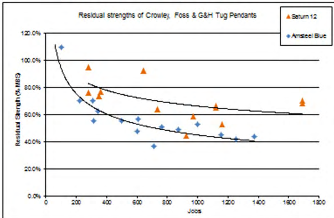
Figure 2.3 Residual Strength Data (Courtesy of Samson Ropes)
