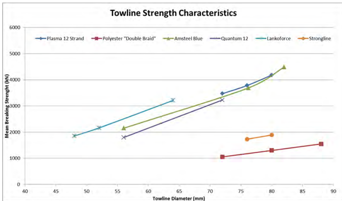
Figure 2.1 Towline Strength Characteristics
