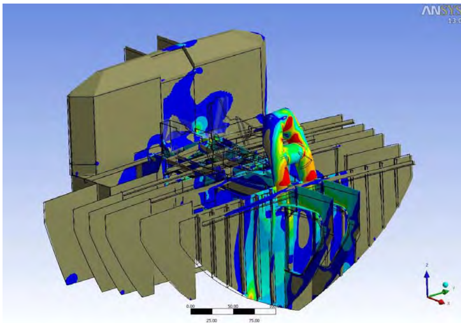
Figure 2.9 FEA Models of Escort Towing Staples:
