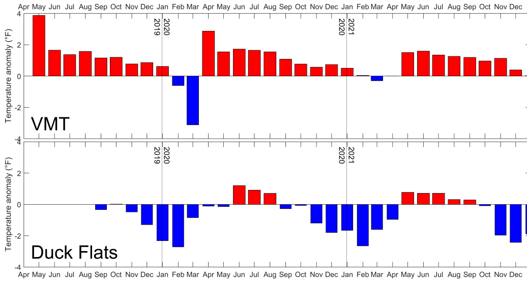
Figure 19: Monthly average air temperature anomalies at the VMT. This is the same data as in figure 18, but scaled to the time period the VMT buoy has been deployed.
