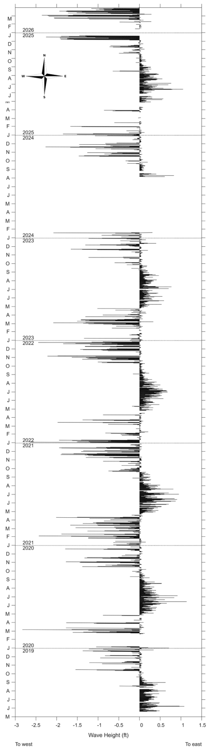
Figure 13: Quiver plot of average daily wave vectors (direction and height in feet) at the VMT buoy. The length of each stick indicates wave height and the angle indicates the direction the waves are travelling in.
