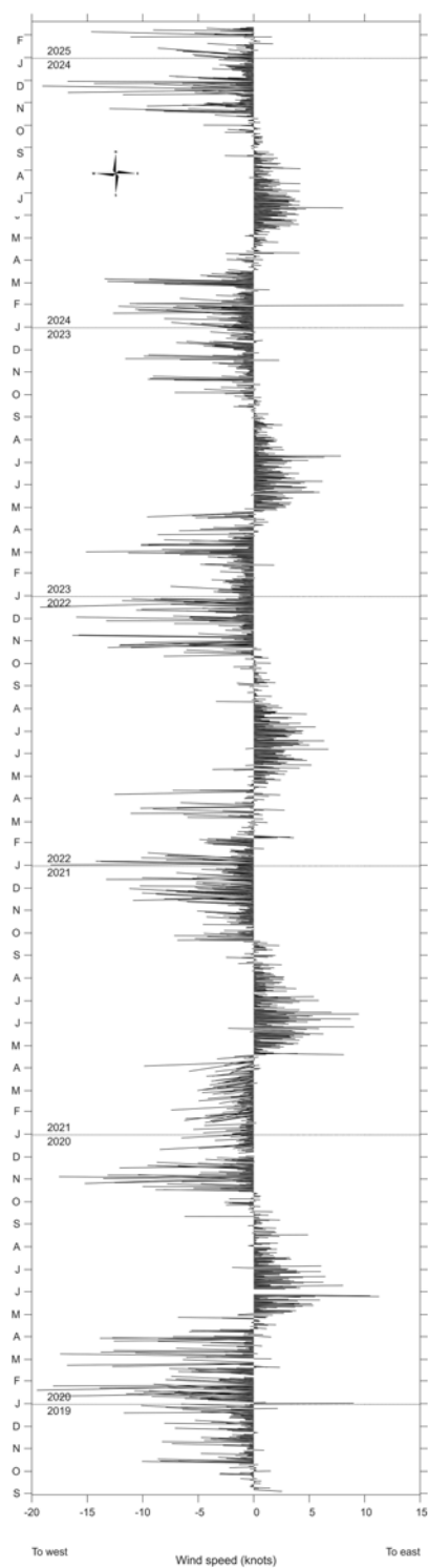
Figure 9: Quiver plot of average daily wind vectors at the Duck Flats buoy. The length of each stick indicates wind speed and the angle indicates the direction from.
