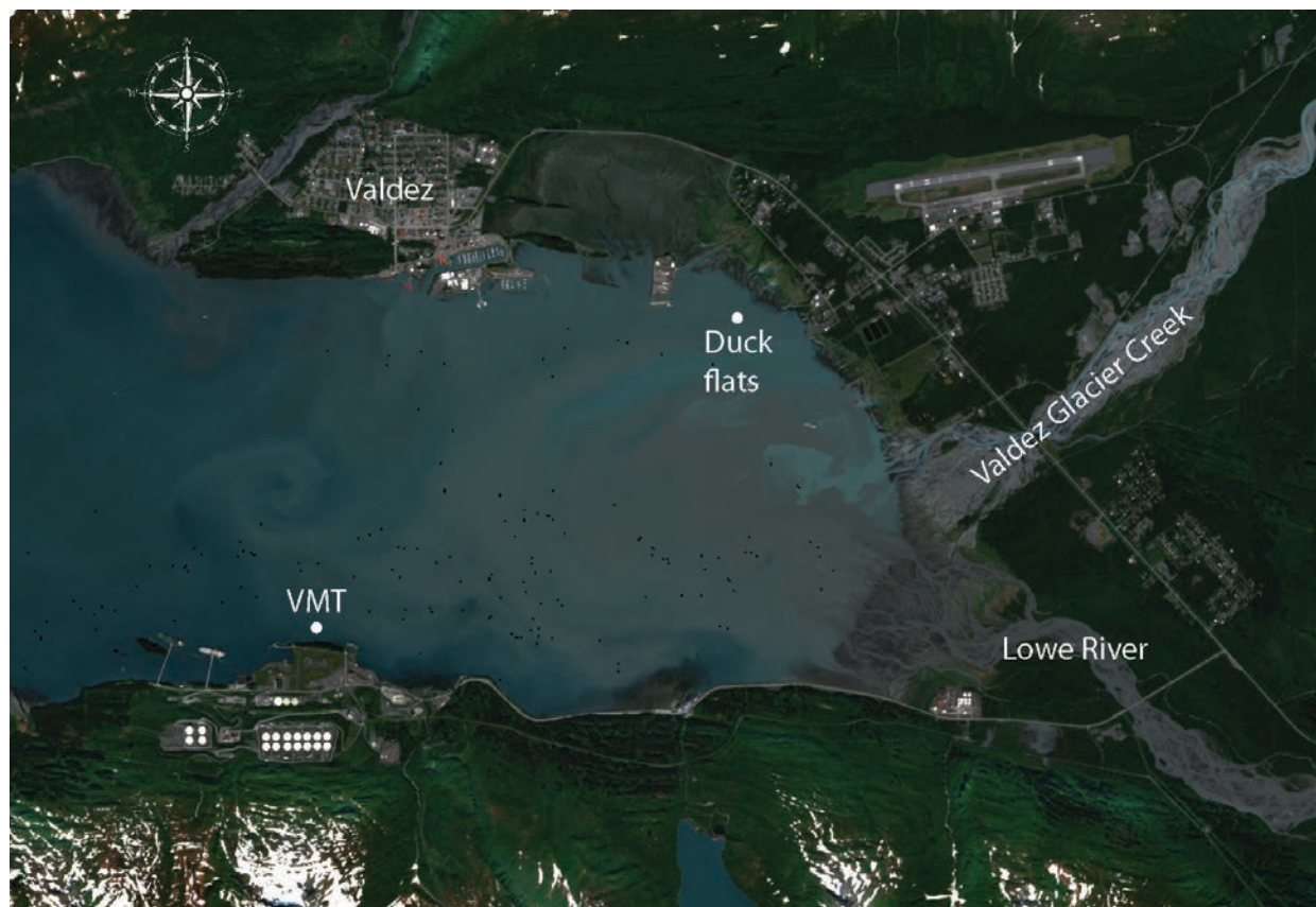
Figure 1: Sentinel 2 satellite image of Port Valdez (taken June 22, 2022) showing the location of the two buoys and other geographic locations mentioned in the report.
