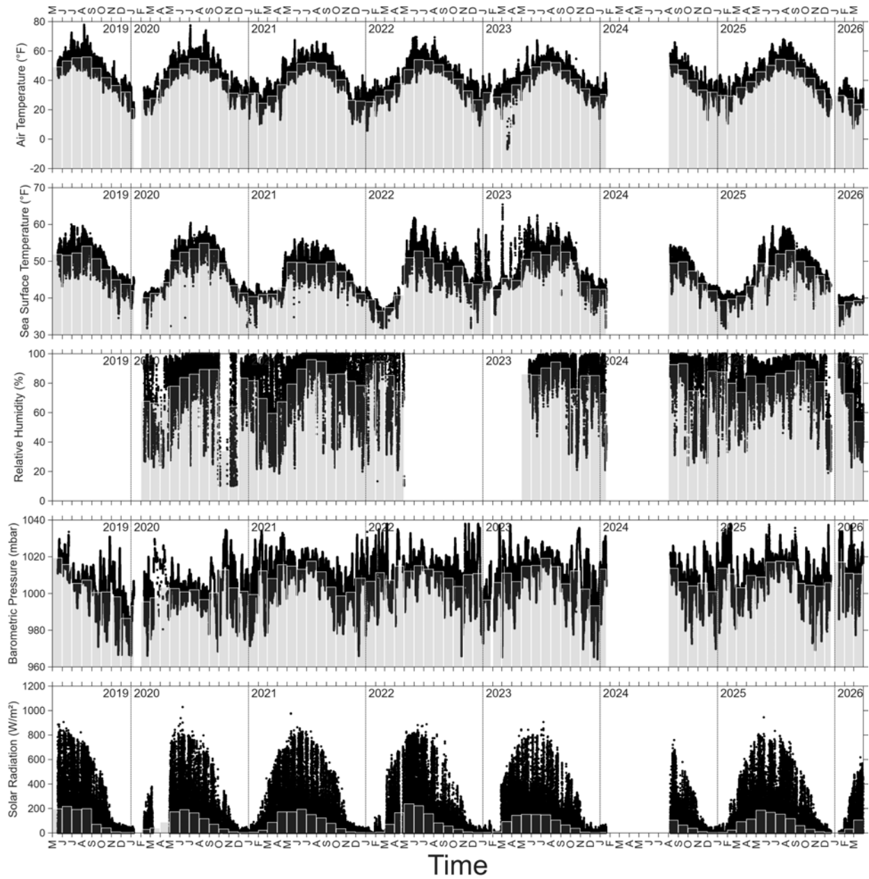
Figure 4: Scalar observations at the VMT buoy, including air (top panel) and water (2 nd panel) temperatures, relative humidity (3 rd panel), barometric pressure (4 th panel), and solar radiation (bottom panel). Black dots are observations, bars indicate monthly averages.
