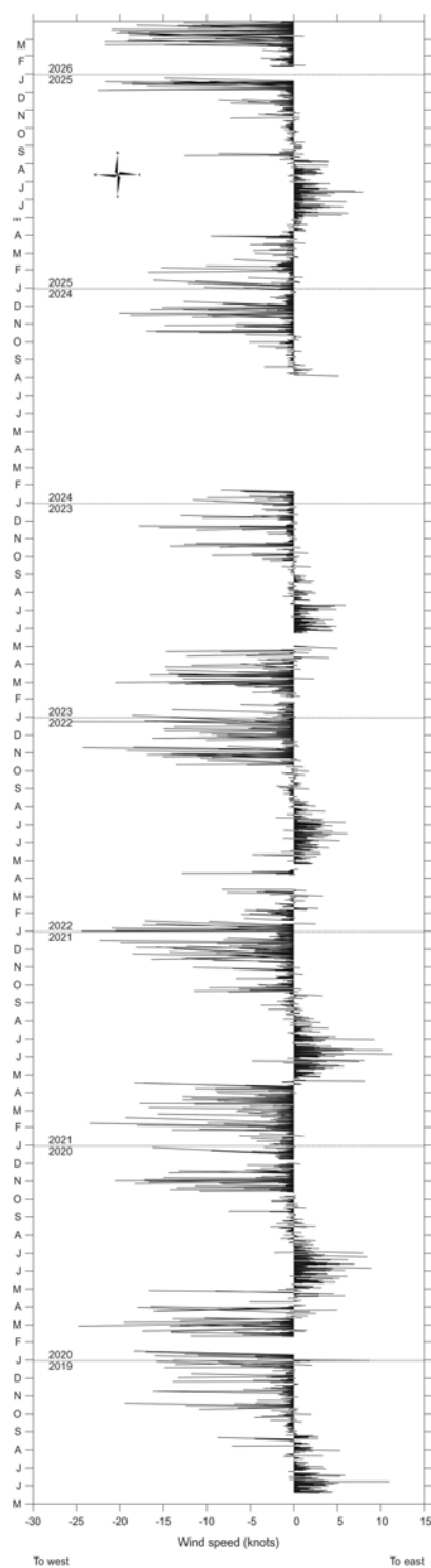
Figure 8: Quiver plot of average daily wind vectors at the VMT buoy. The length of each stick indicates wind speed and the angle indicates the direction from.
