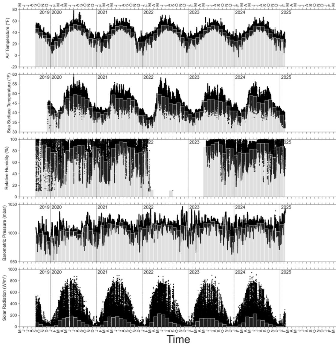
Figure 5: Scalar observations at the Duck Flats buoy, including air (top panel) and water (2 nd panel) temperatures, relative humidity (3 rd panel), barometric pressure (4 th panel), and solar radiation (bottom panel). Black dots are observations, bars indicate monthly averages.
