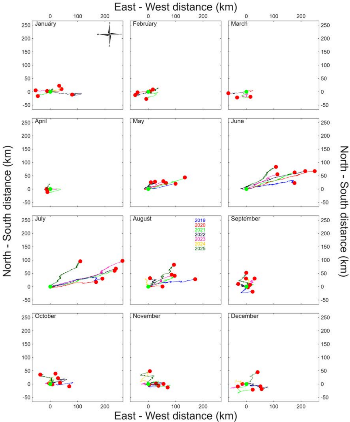
Figure 21: Monthly PVD of surface currents at the VMT buoy, 2019-2025. All axes are scaled to be the same to make each vector track comparable. The bottom axis indicates direction east-west, with westerly directions negative and easterly ones positive, the side axis indicates direction north-south, with southerly directions negative.
