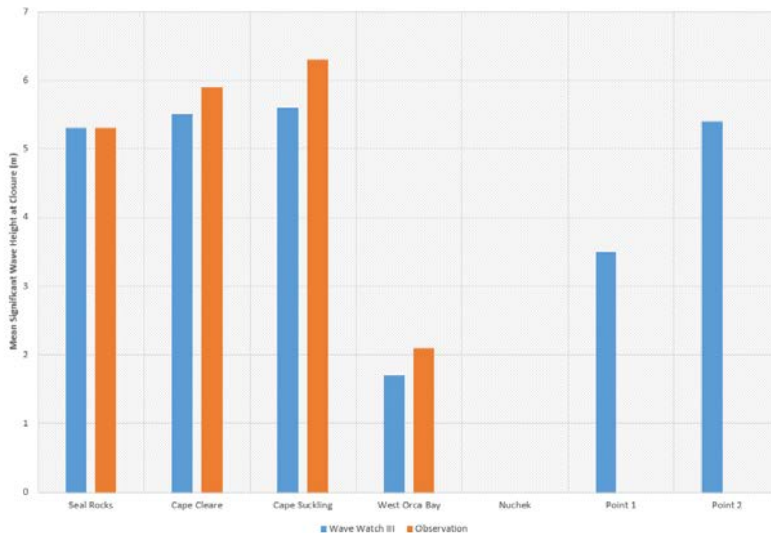
Mean Significant Wave Height (m) Simulated by Wave Watch III and Observed
