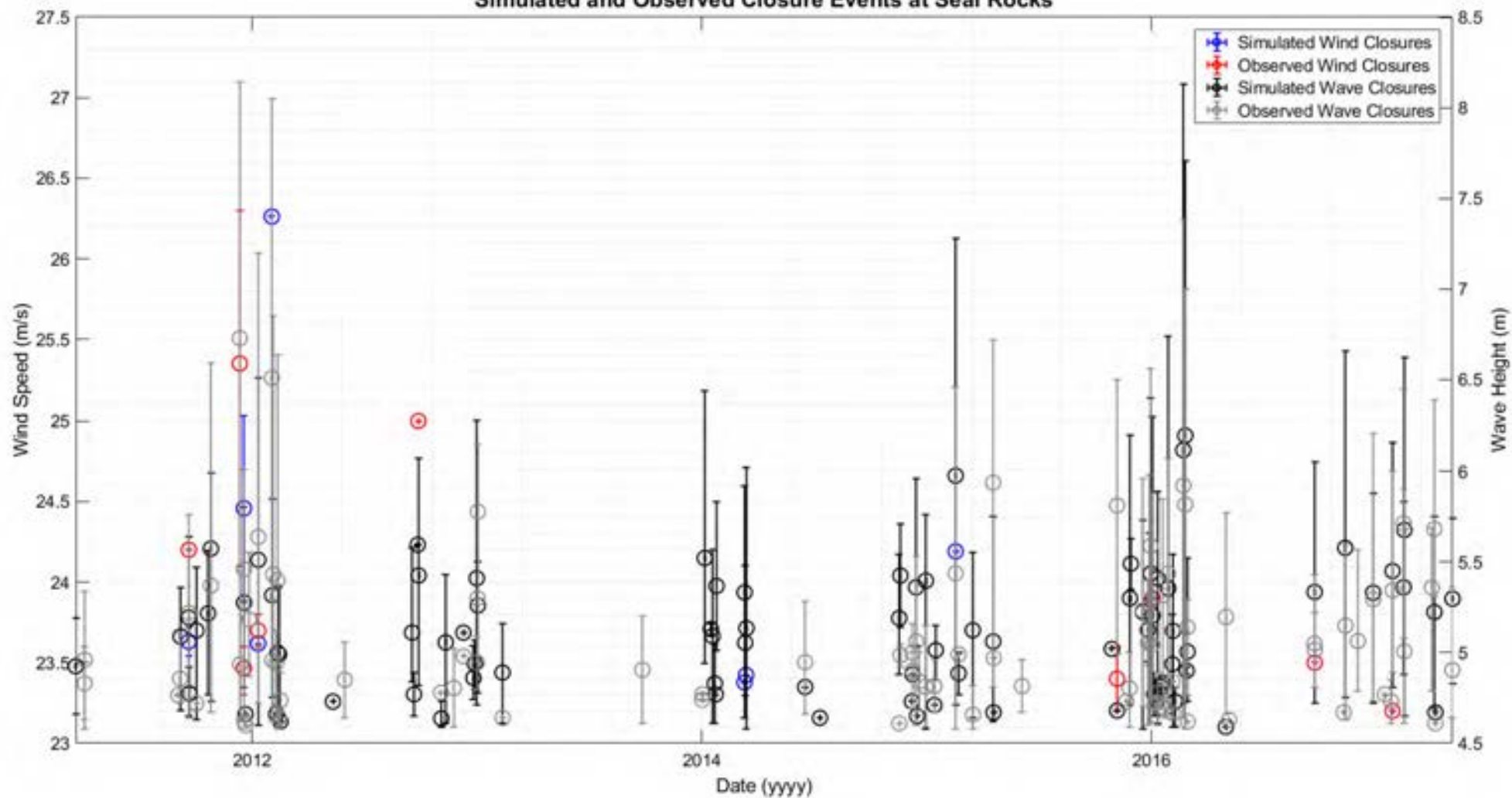
Simulated and Observed Closure Events at Seal Rocks
