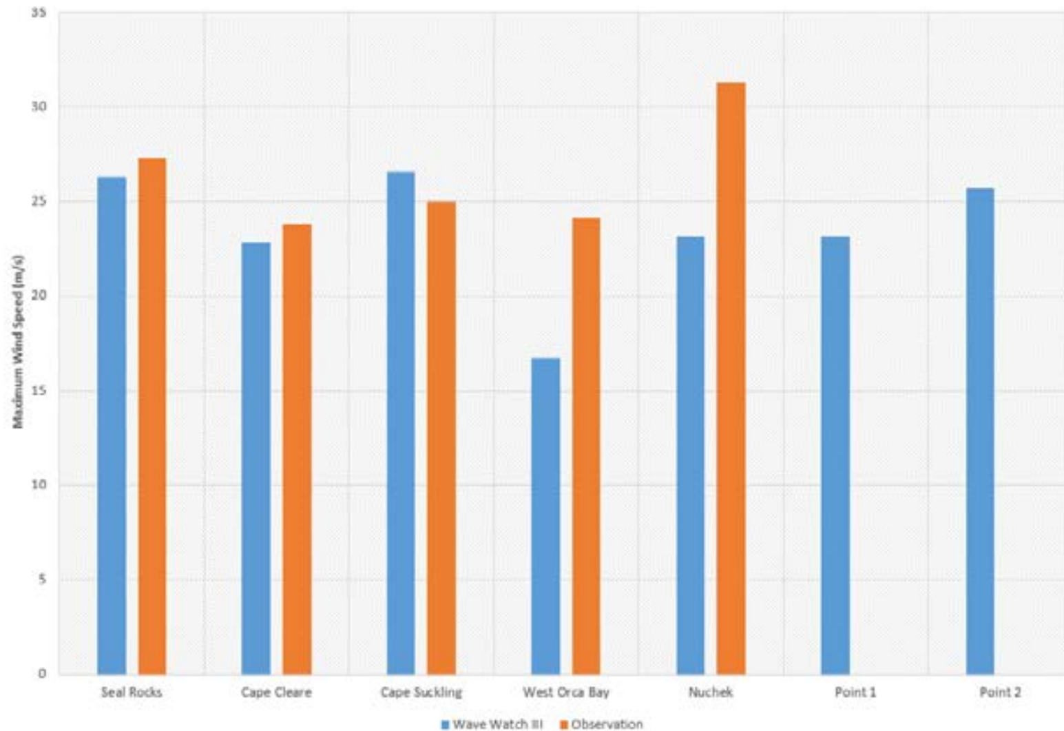
Maximum Wind Speed (m/s) Simulated by Wave Watch III and Observed
