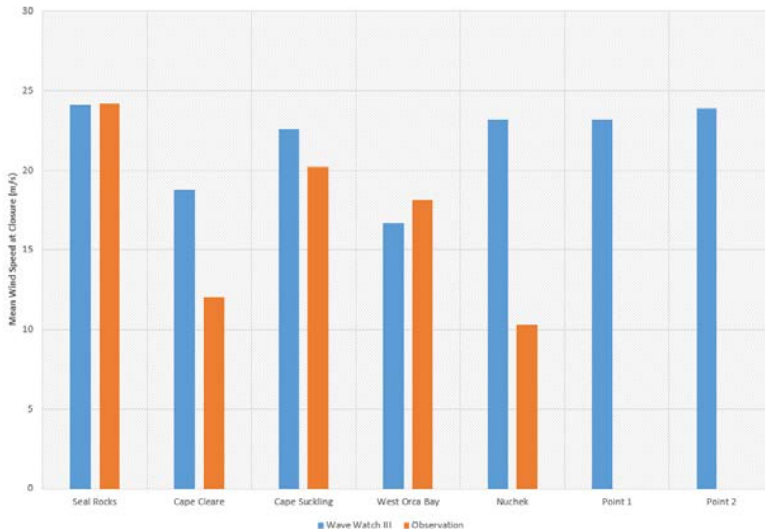
Mean Wind Speed at Closure (m/s) Simulated by Wave Watch III and Observed
