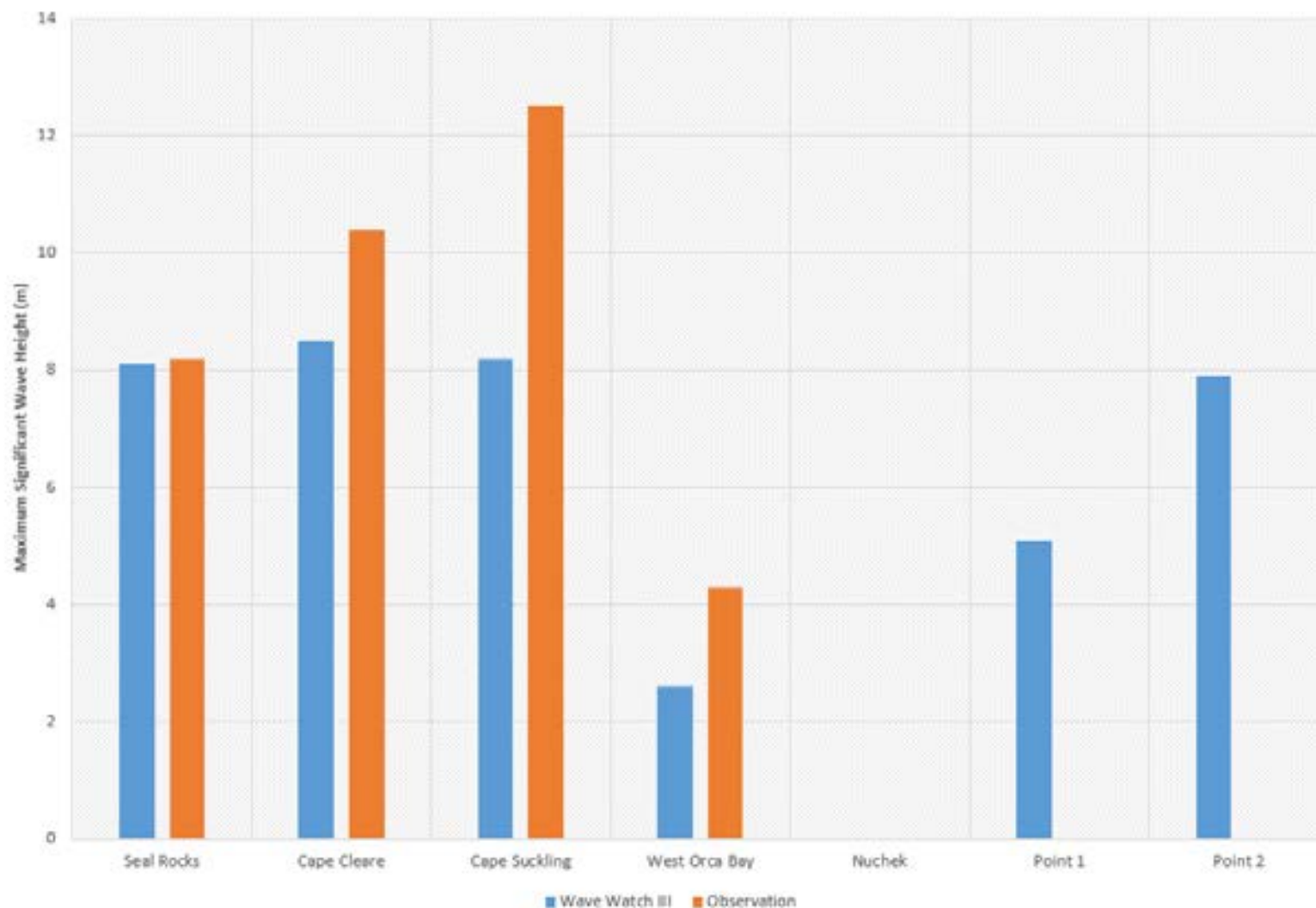
Maximum Significant Wave Height (m) Simulated by Wave Watch III and Observed
