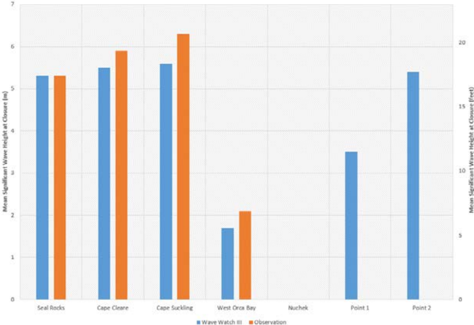
Mean Significant Wave Height (m) Simulated by Wave Watch III and Observed
