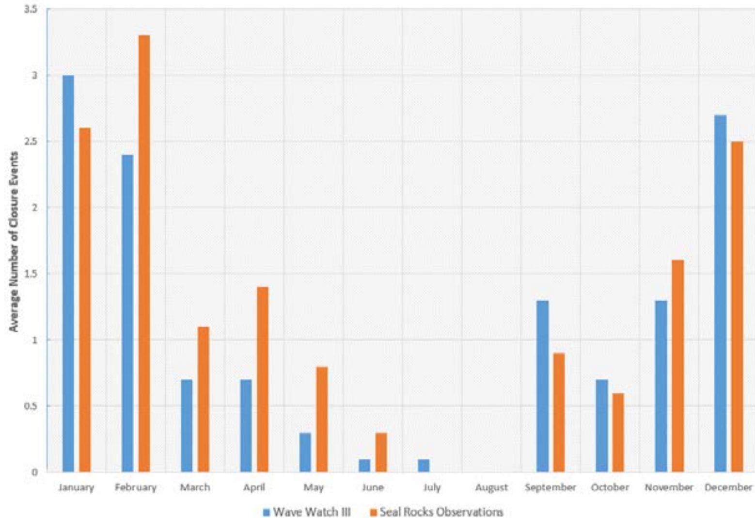
Simulated and Observed Average Number of Closure Events Per Month
