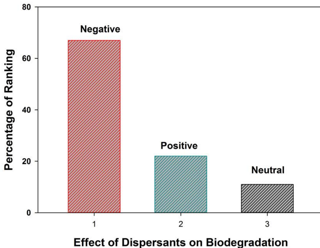
Figure 2 The ratings of the detailed studies as to the effect that chemical dispersion had on biodegradation. Sixty-seven percent of studies showed inhibition of degradation, 22% as promoting biodegradation and 11% as having mixed or neutral effects.
