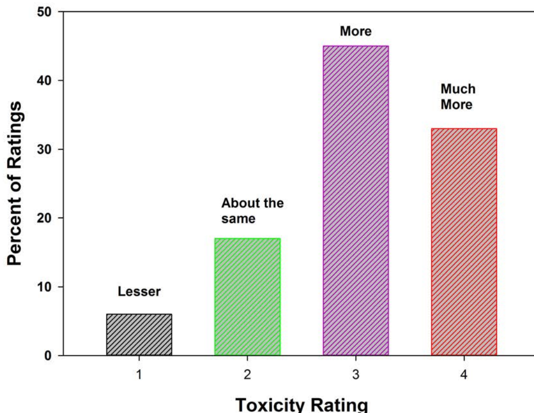
Figure 1 A summary of the toxicity ratings as graded in this review. This indicates that most of the studies reviewed found that most of the time the toxicity of the chemically-dispersed oil was greater than that of the mechanically-dispersed oil.
