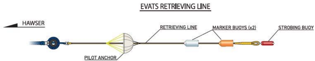
Figure 10 Samson, EVATS™ Retrieving Line assembly
